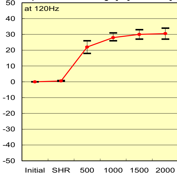
Capacitance Change[%] vs Time[h]
