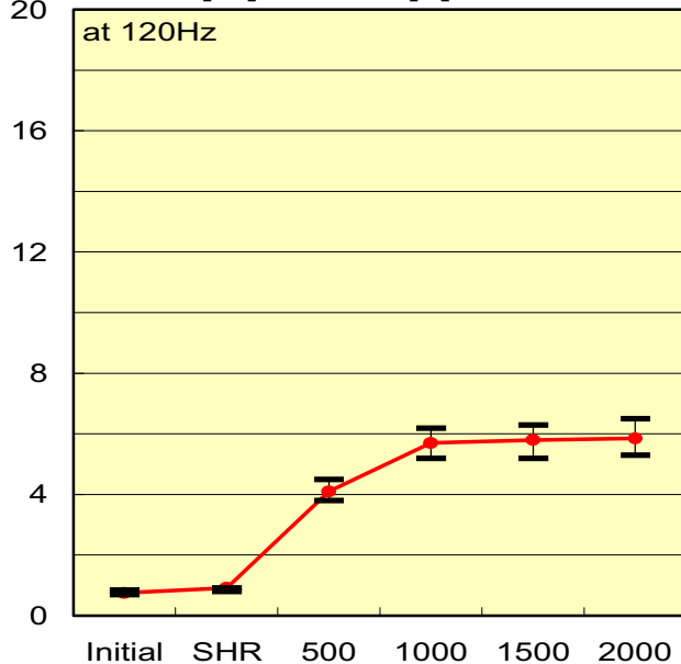
tan δ [%] vs Time[h]
