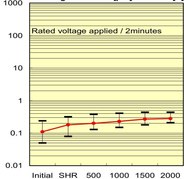
Leakage Current [μA] vs Time[h]
