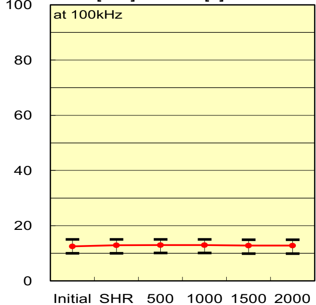
ESR [mΩ] vs Time[h]
