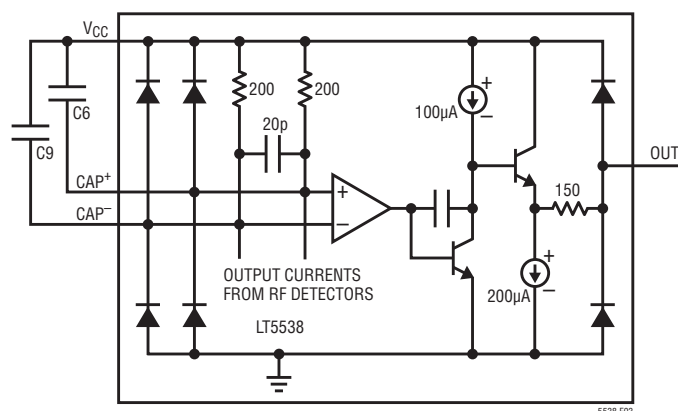
Figure 3. Simplified Schematic of the Output Interface
