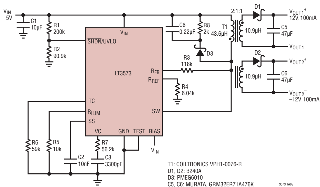
\pm 12\text{V} Isolated Flyback Converter
