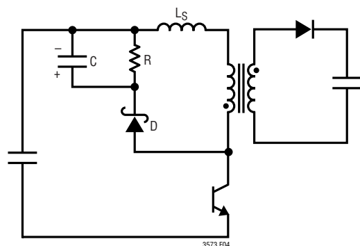
Figure 4. RCD Clamp
