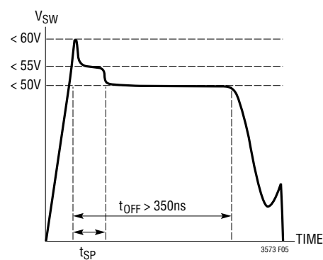
Figure 5. Maximum Voltages for SW Pin Flyback Waveform
