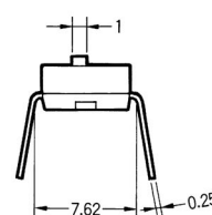
Raised Actuator
