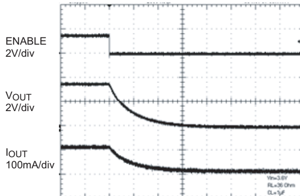
Turn-Off Timing
