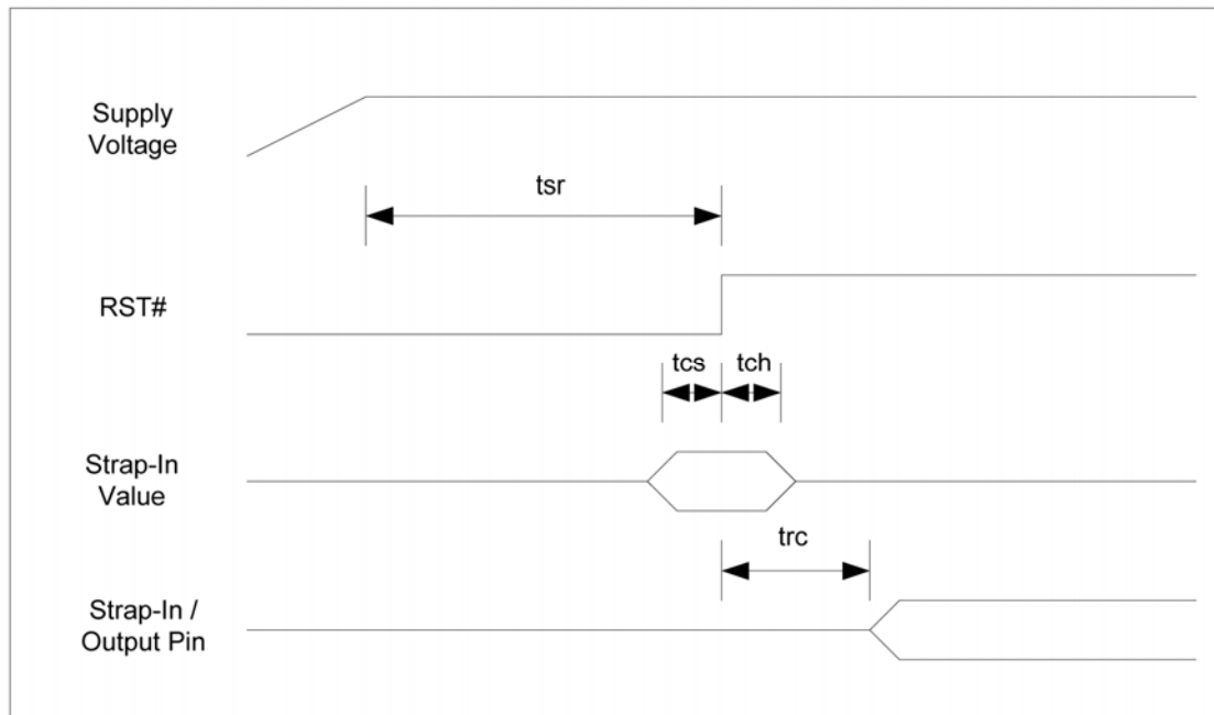
Figure 18. Reset Timing
