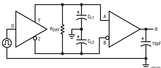
Figure 3. Driver/Receiver Timing Test Load
