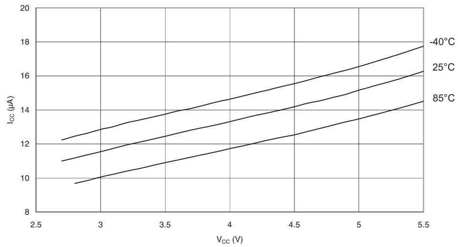
Figure 207. ADC Current vs. V_{CC} (Aref = AVCC)
