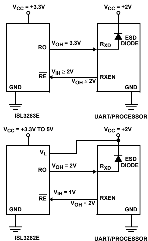
FIGURE 6. USING V L PIN TO ADJUST LOGIC LEVELS
