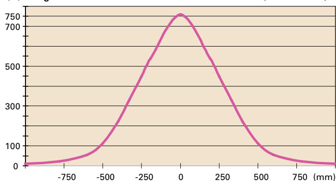
(lx) Light Distribution at 0.5m LF1A-D1-THWW6 (Cool White)
