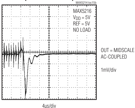
MAJOR CODE TRANSITION (0x3FFF TO 0x8000)
