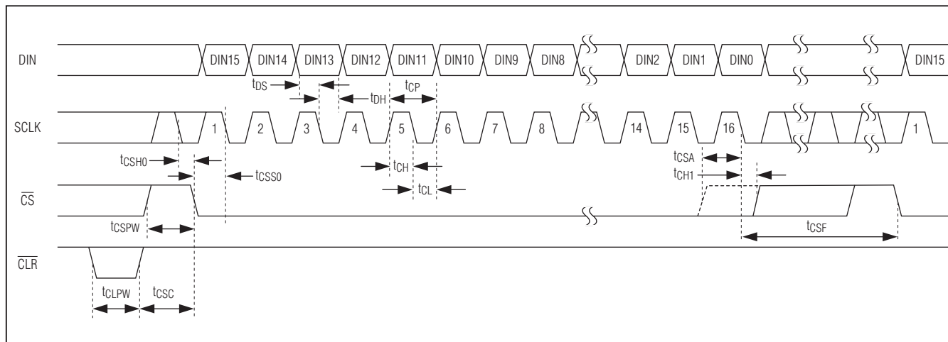
Figure 1. 16-Bit Serial-Interface Timing Diagram (MAX5214)
