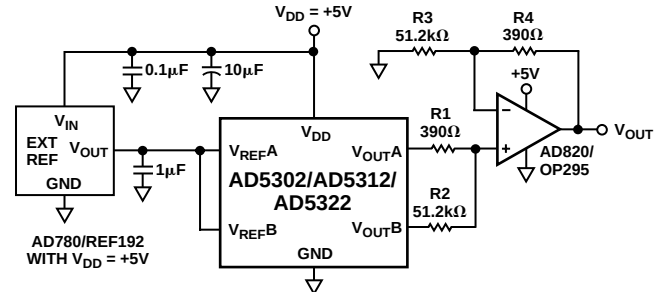
Figure 42. Coarse/Fine Adjustment
