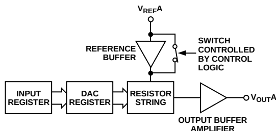
Figure 26. Single DAC Channel Architecture
