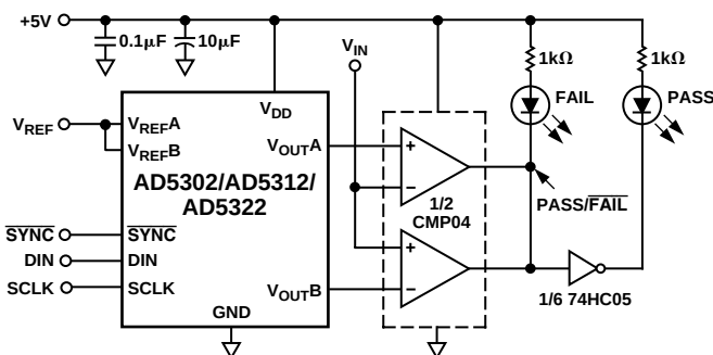
Figure 41. Window Detector Using AD5302/AD5312/AD5322
