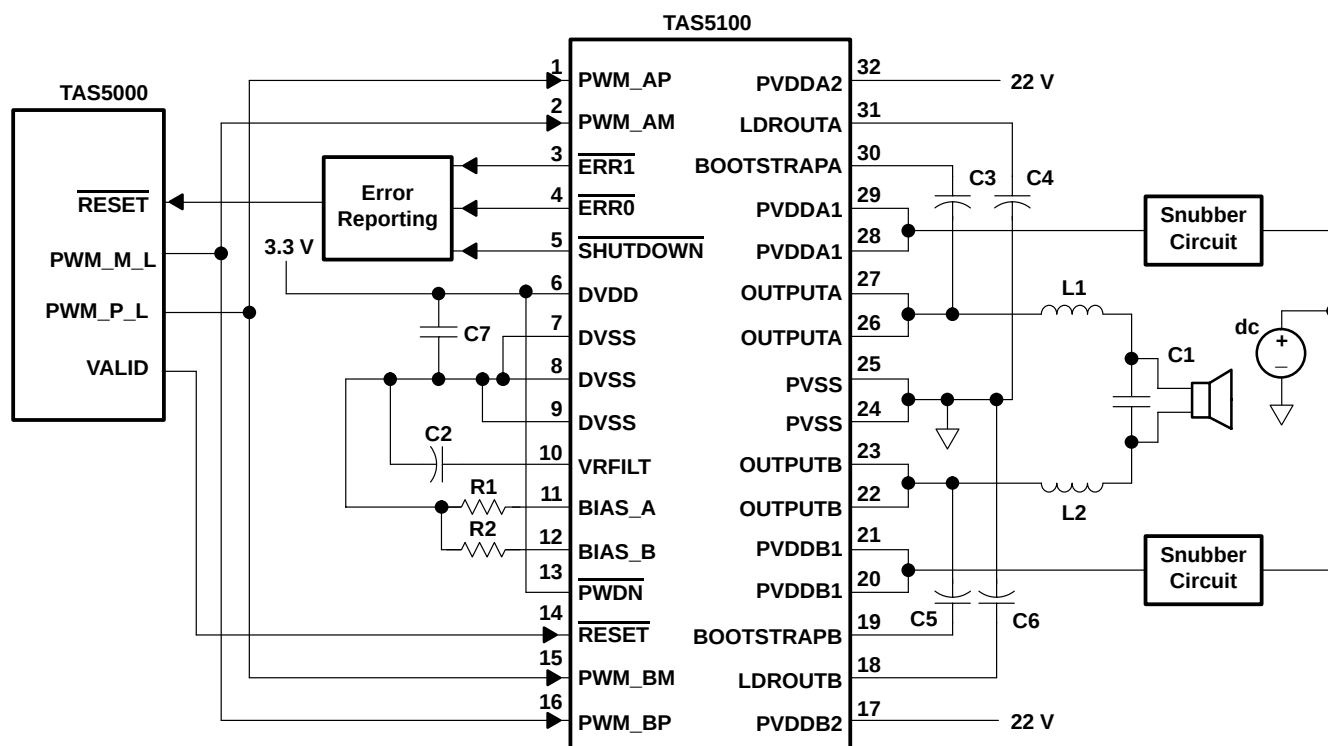
Figure 5. Typical TAS5100 Application (One Channel Shown)
