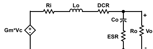
FIGURE 7. THE EQUIVALENT CIRCUIT OF THE POWER STAGE WITH CURRENT LOOP INCLUDED
