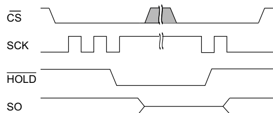
Figure 27. \overline{HOLD} Operation
