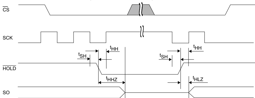
Figure 30. HOLD Timing
