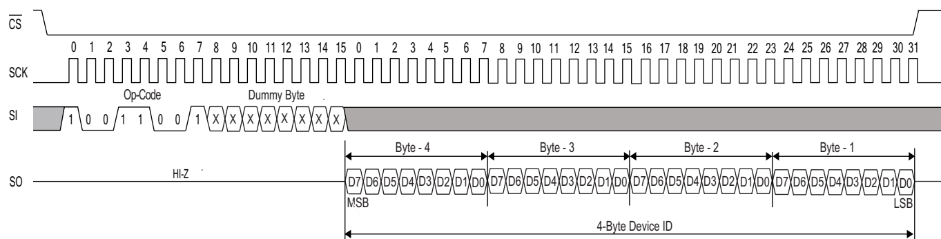
Figure 26. FAST_RDID instruction
