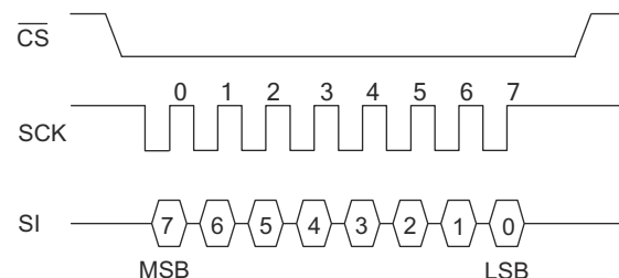
Figure 6. SPI Mode 3
