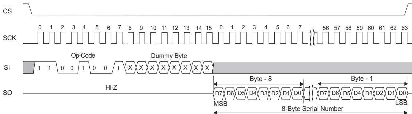
Figure 24. FAST_RDSN Instruction
