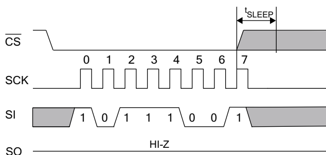
Figure 22. WRSN Instruction
