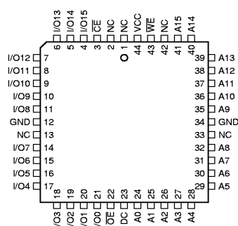
PLCC Top View
