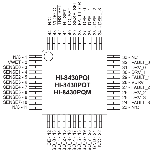
44 - Pin Plastic Quad Flat Pack (PQFP) 10mm x 10mm body
