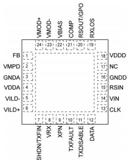
24-Pin MLF®
