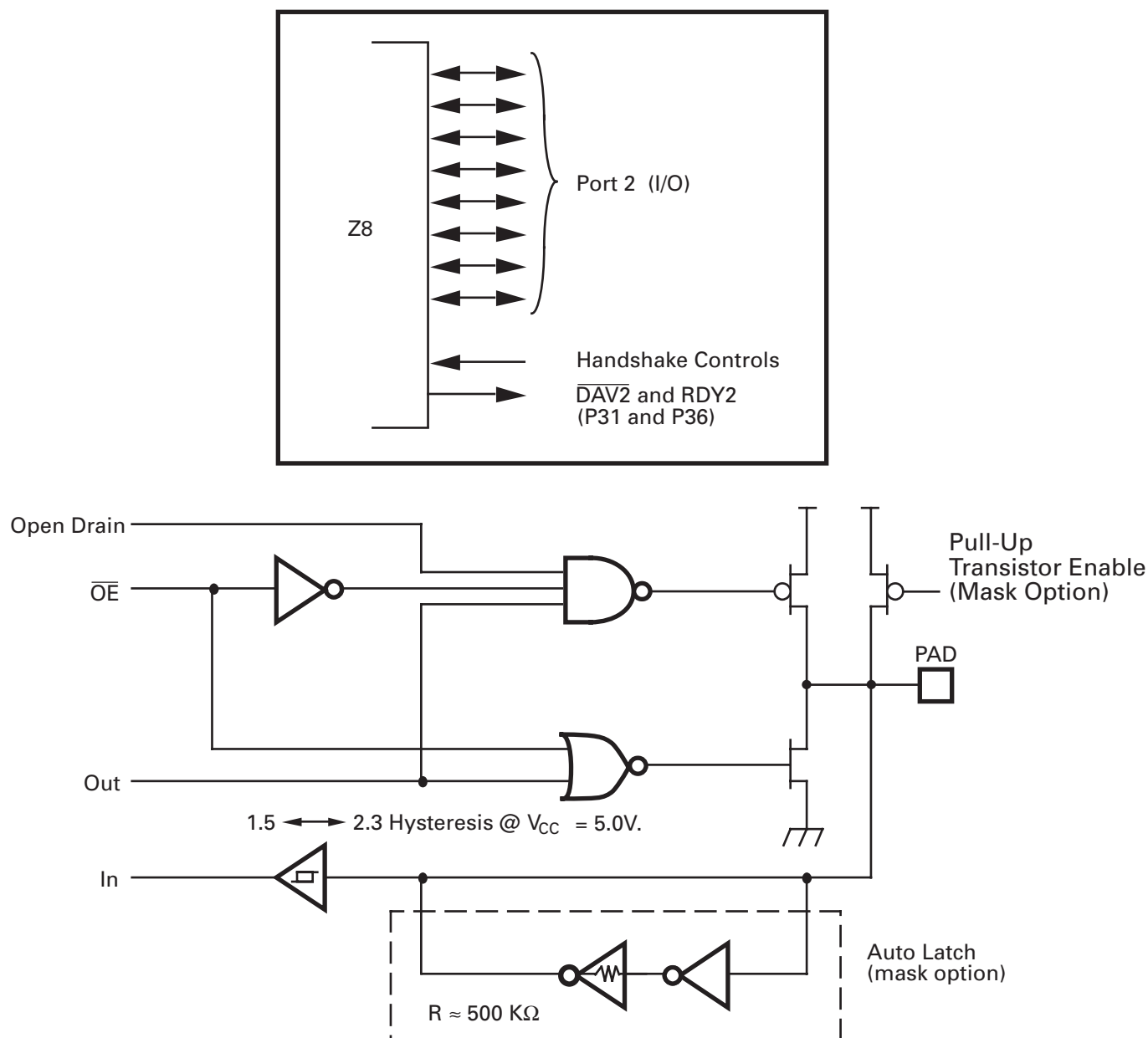
Figure 14. Port 2 Configuration
