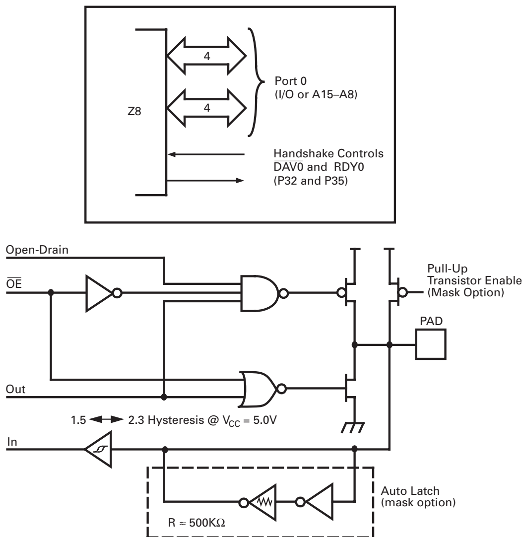
Figure 12. Port 0 Configuration
