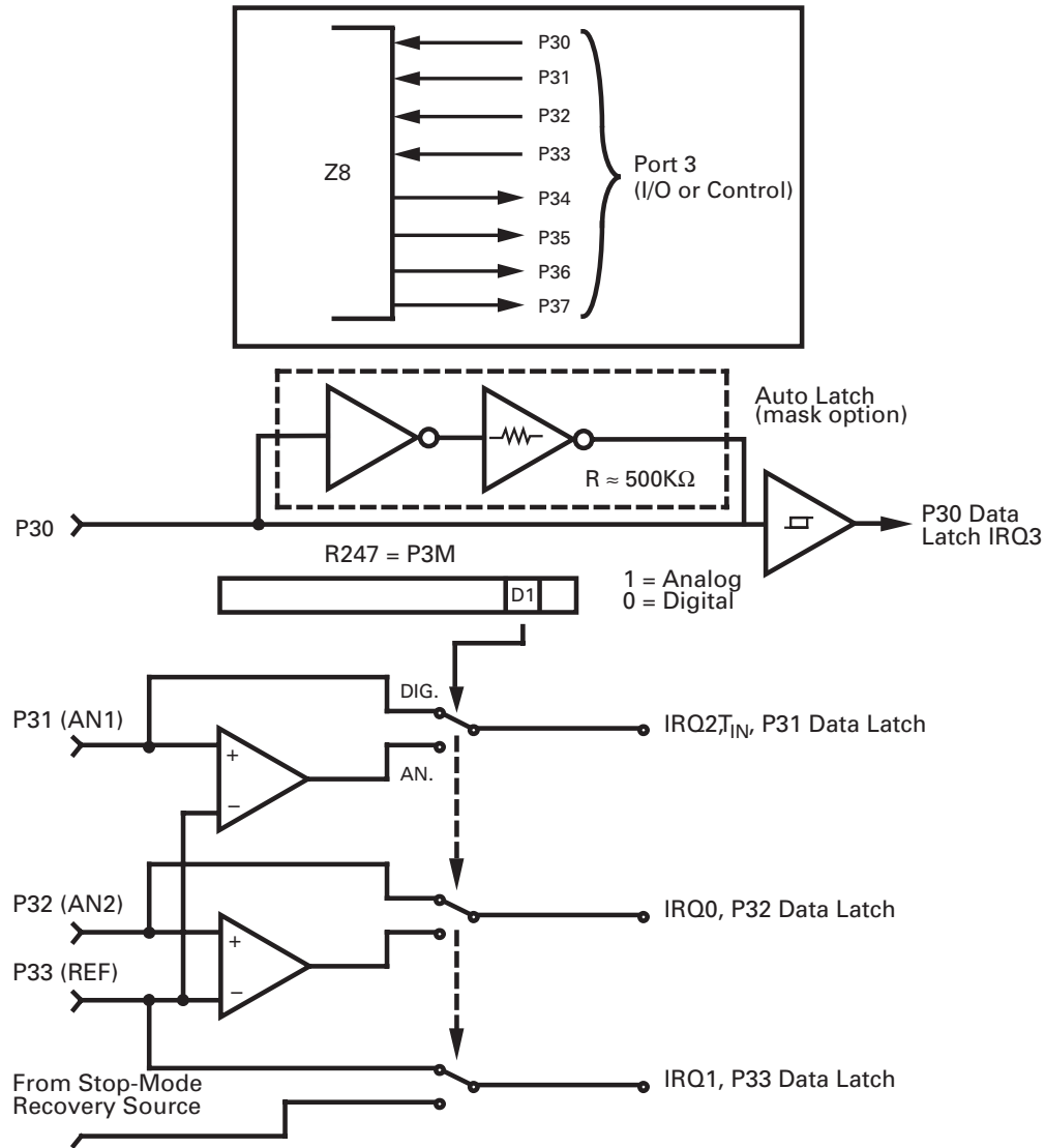
Figure 15. Port 3 Configuration
