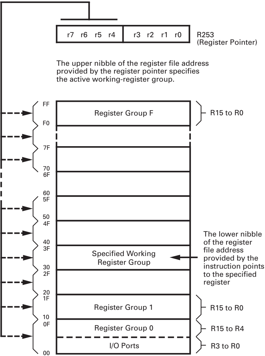
Figure 21. Register Pointer—Detail
