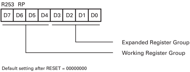
Figure 20. Register Pointer
