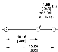
Recommended Mounting Hole Layout
