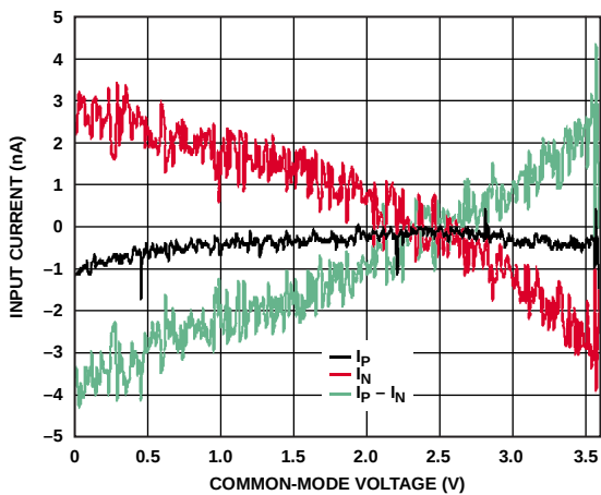
Figure 10. Input Current vs. Common-Mode Voltage ( V_{CM} ), Gain = 128, ADC Input = 7.8125 mV, AVDD = 3.6 V, T_A = 25^\circ\text{C} , V_{CM} = ((AIN+) + (AIN-))/2
