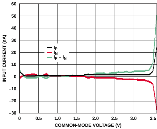
Figure 9. Input Current vs. Common-Mode Voltage ( V_{CM} ), Gain = 4, ADC Input = 250 mV, AVDD = 3.6 V, T_A = 25^\circ\text{C} , V_{CM} = ((AIN+) + (AIN-))/2
