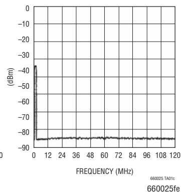
LT6600-2.5 Output Spectrum
