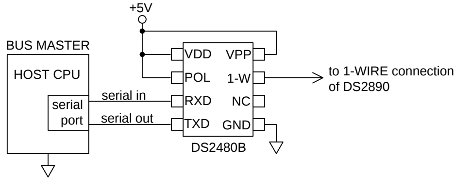
FIGURE 15. BUS MASTER WITH DS2480B DRIVER
