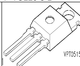
P-TO220-3-1
