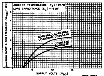
Fig. 12 - Maximum input clock frequency vs. V_{DD} .
