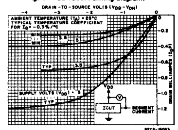
Fig. 5 - Minimum and typical output p-channel decoded drain characteristics @ V_{DD}=3.5 & 5 V.
