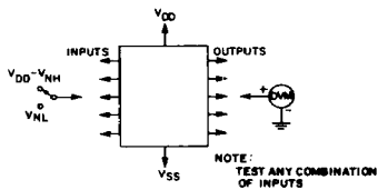
Fig. 14 - Noise immunity test circuit.
