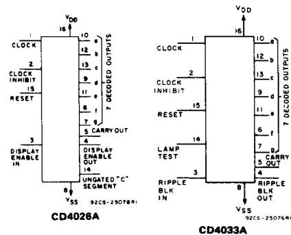
FUNCTIONAL DIAGRAMS
