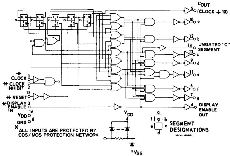
Fig. 1 - CD4026A logic diagram.
