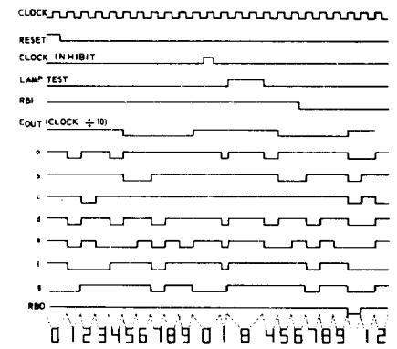
Fig. 4 - CD4033A timing diagram.
