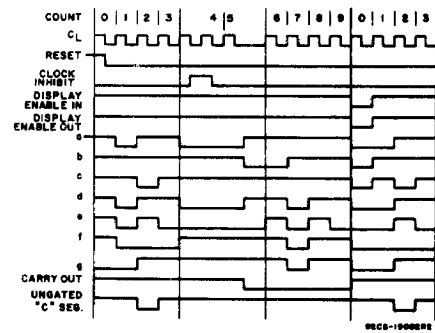
Fig. 2 - CD4026A timing diagram.
