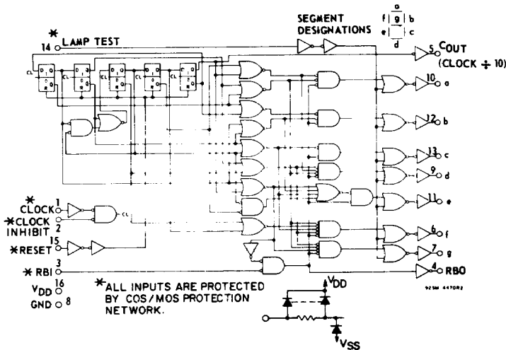
Fig. 3 - CD4033A logic diagram.
