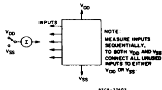
Fig. 16 - Input-leakage-current test circuit.
