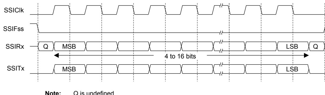
Figure 12-6. Freescale SPI Frame Format with SPO=0 and SPH=1
