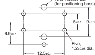
PCB Mounting (Top View) (Single-sided PCB, t=1.6 )
