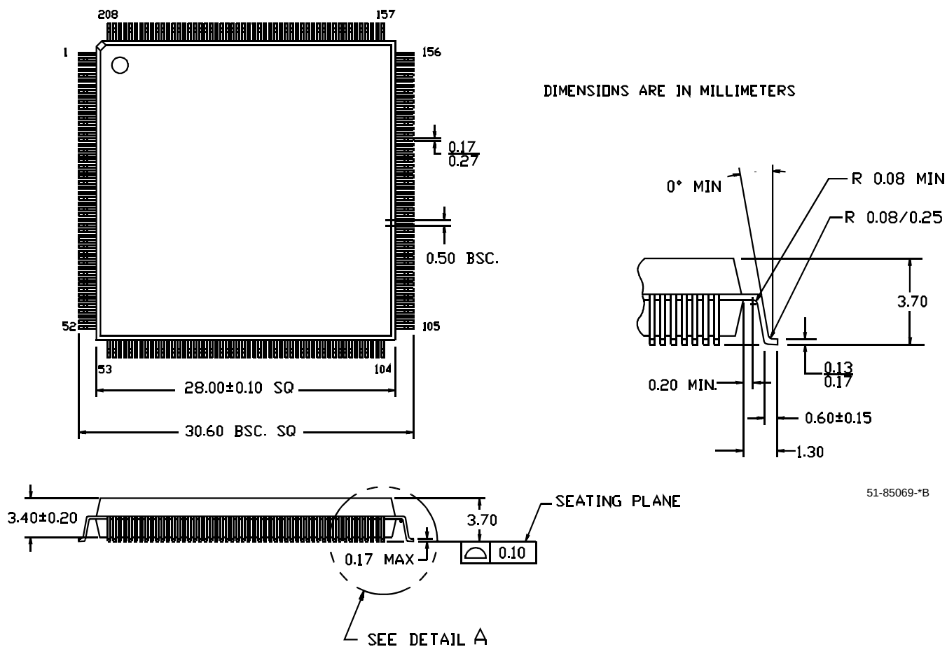
208-Lead Enhanced Quad Flat Pack (EQFP) NT208
