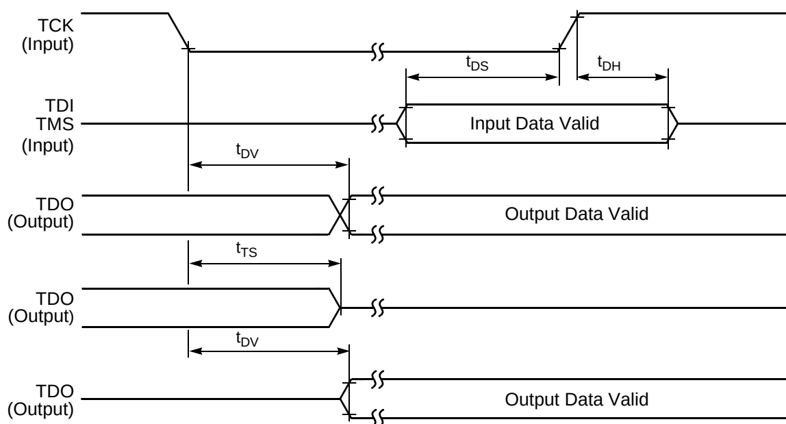
Figure 3-29 Test Access Port Timing Diagram
