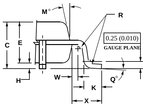
Figure 4-2 100-pin LQPF Mechanical Information
