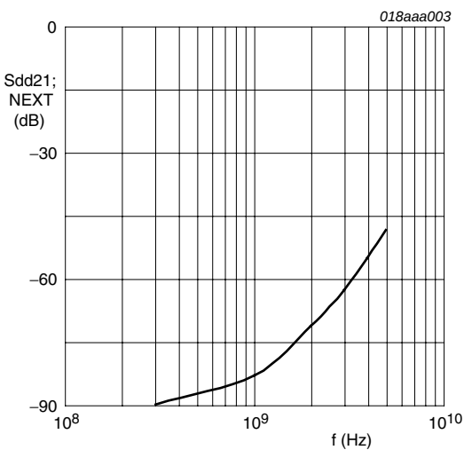
Sdd21 normalized to 100 \Omega ; differential pairs CH1/CH2 versus CH3/CH4
