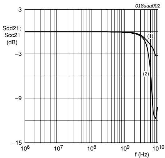
(1) Sdd21 (2) Scc21 normalized to 100 \Omega ; differential pairs at CH1/CH2 or at CH3/CH4
