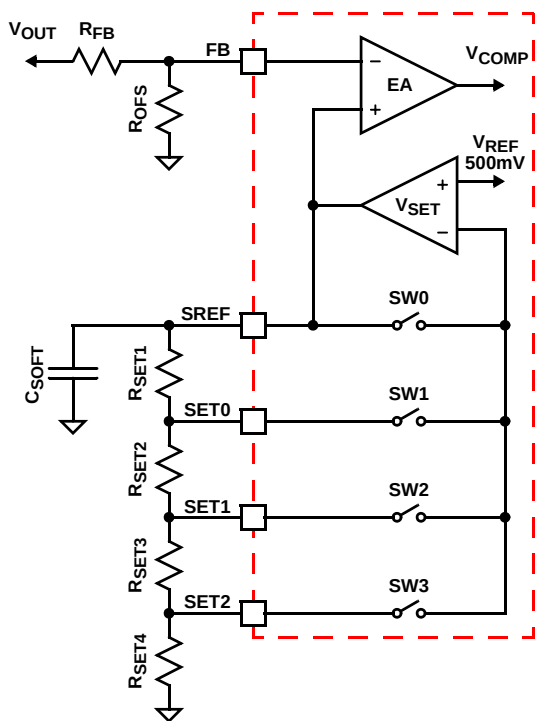
FIGURE 8. ISL62872 VOLTAGE PROGRAMMING CIRCUIT
