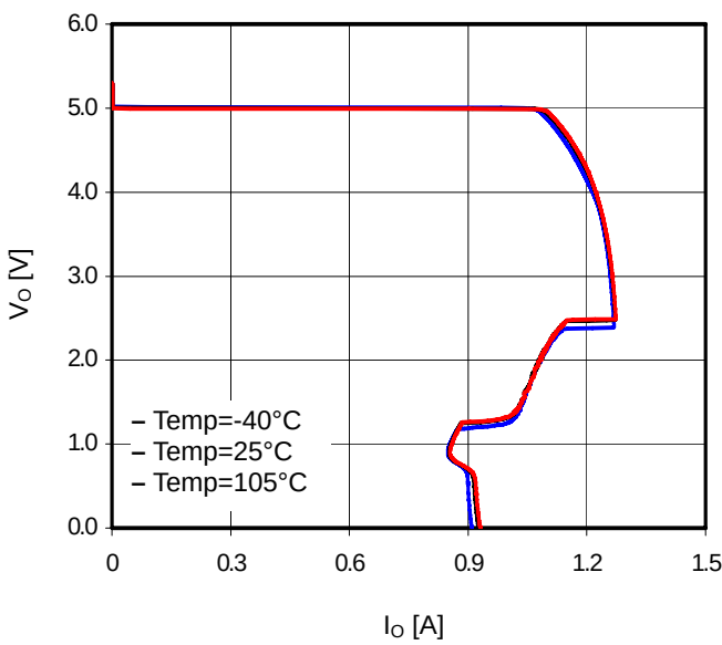
Figure 29. OCP
