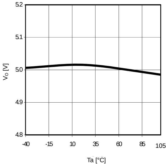
Figure 21. T_a - V_O ( I_o = 0\text{mA} )
