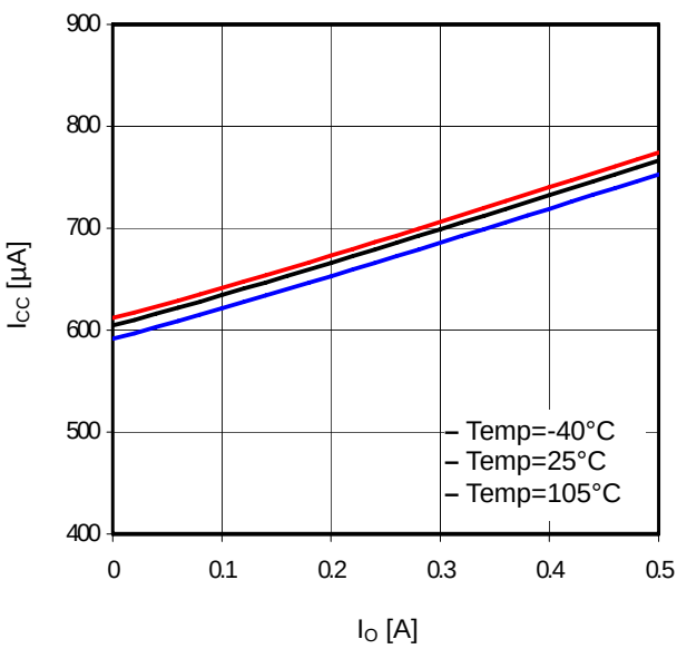
Figure 30. I_o-I_{CC}
