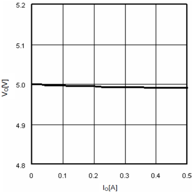
Figure 25. I_O - V_O
