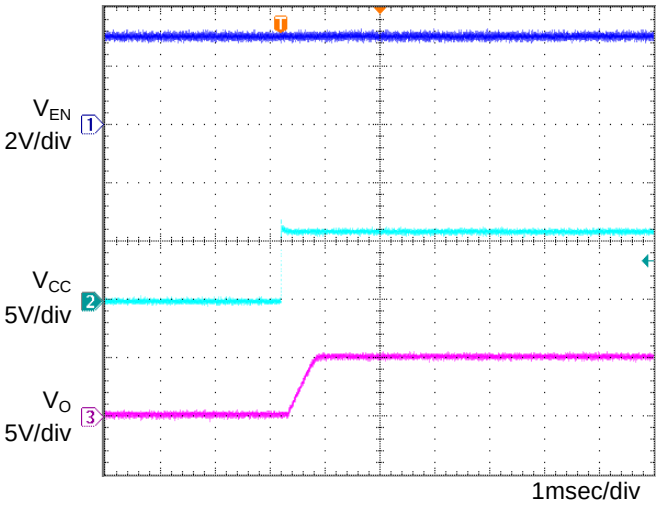
Figure 10. Input sequence 1 C_o=1\mu F , T_a=25^{\circ}C
