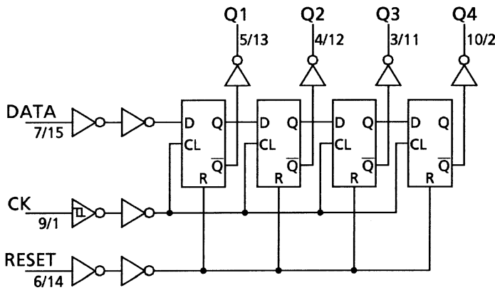
1/2 TC4015B
