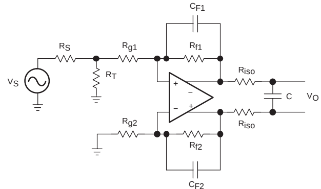
A Two-Pole, Low-Pass Filter Design Using a Fully Differential Amplifier With Poles Located at:
