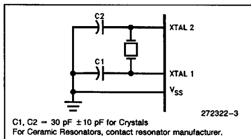
Figure 3. Oscillator Connections
