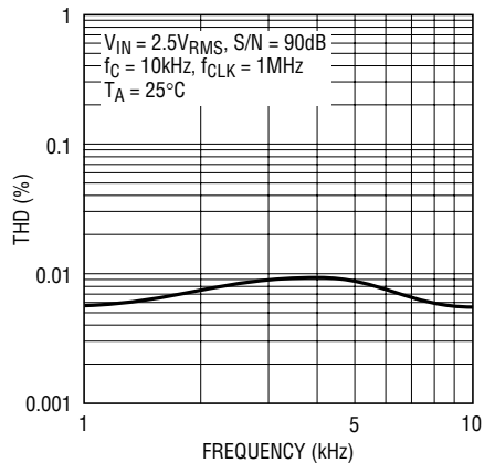
THD vs Frequency; V_S = \pm 7.5\text{V}
