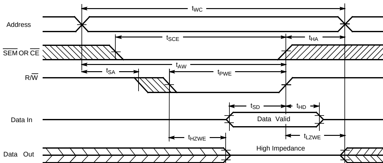
Figure 9. Write Cycle No. 2: \text{R}/\overline{\text{W}} Three-State Data I/Os (Either Port) [19, 21, 22]
