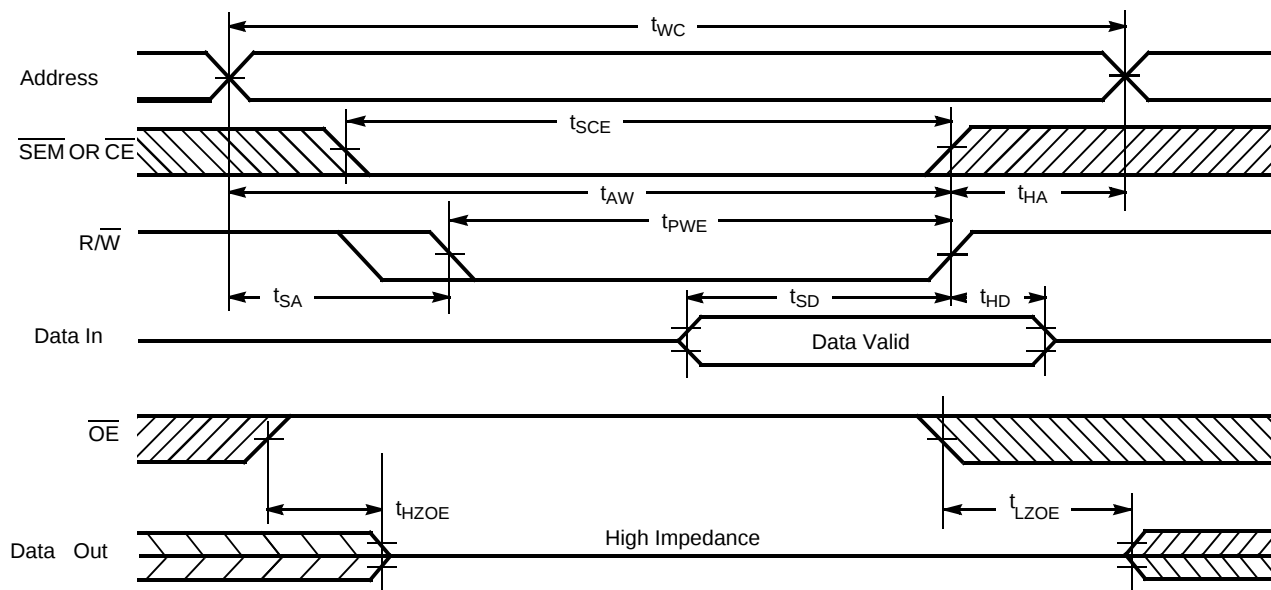
Figure 9. Write Cycle No. 2: \text{R}/\overline{\text{W}} Three-State Data I/Os (Either Port) [19, 21, 22]
