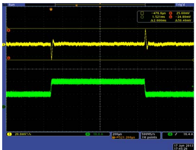
FIGURE 14. STEP RESPONSE, 10A TO 20A @ 5A/ \mu s, ASCR = 400 TOTAL DEVIATION WINDOW 50mV = 5%
