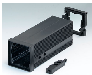
B6012061 DIN-MODULAR CASE TYPE A PPO (UL 94 V-0) black RAL 9005 1.89"x1.89"x4.88"
