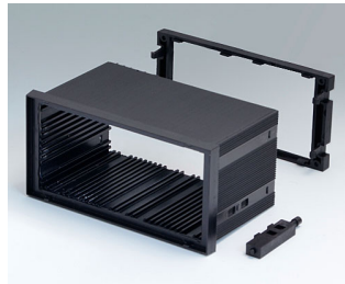
B6043021 DIN-MODULAR CASE TYPE A PPO (UL 94 V-0) black RAL 9005 5.67"x2.83"x2.95"
