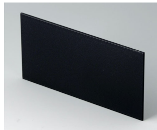
B6143222 Rear panel PPO (UL 94 V-0) black RAL 9005 4.69"x2.47"x0.08"
