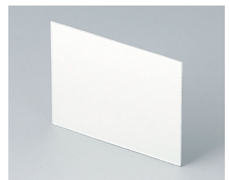
B6123112 Rear panel Aluminum matt anodized 2.51"x1.93"x0.04"
