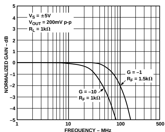
Figure 7. Frequency Response; G = -1, -10 ; V_S = \pm 5\text{ V}
