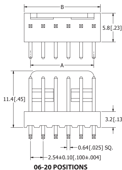
SWR25X-NRTC-S-RA-BA (TYPE 2)
