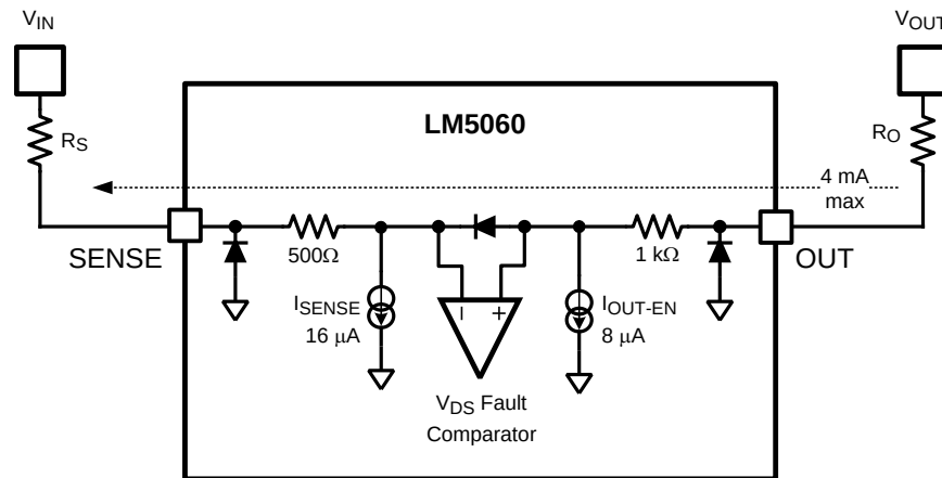
Figure 36. Current Limiting Resistor in the OUT Path for OUT > SENSE Condition
