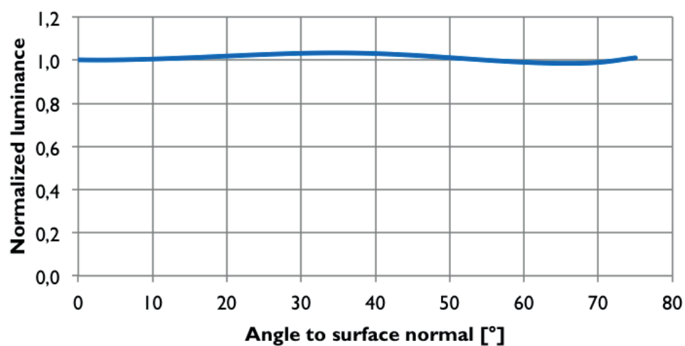
Luminance versus angle
