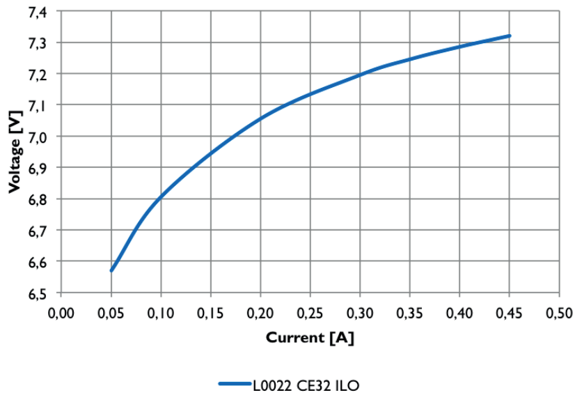
Forward current versus forward voltage
