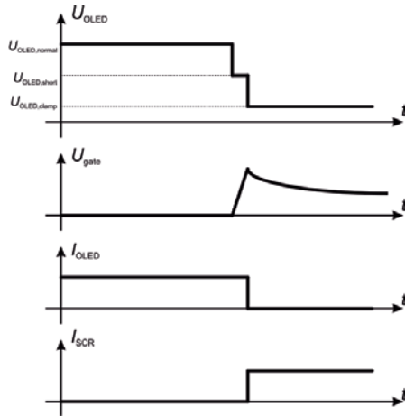
Figure 2: Idealized typical waveforms of the separate failure detection circuit.
