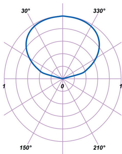
Normalized luminous intensity versus angle
