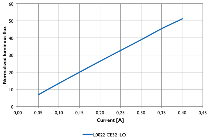
Luminous flux versus forward current
