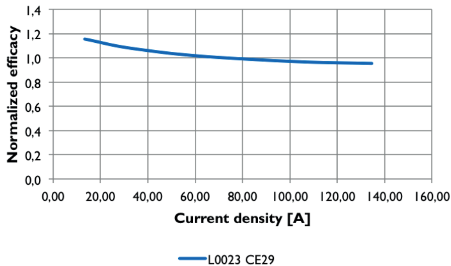
Luminous efficacy versus current density
