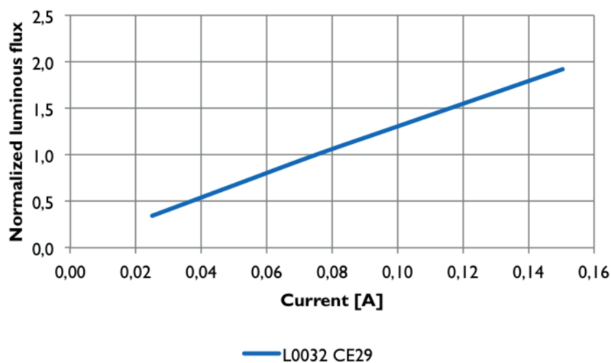
Luminous flux versus forward current
