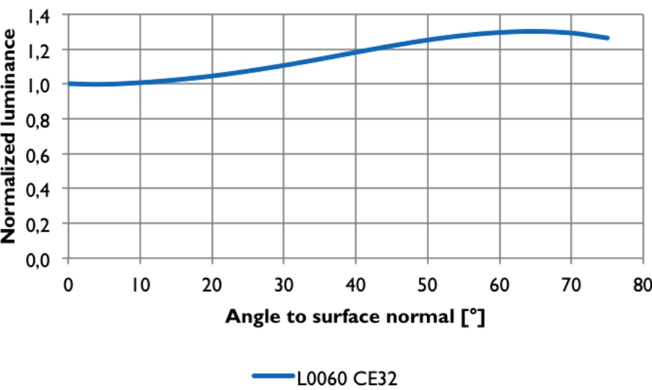
Luminance versus angle
