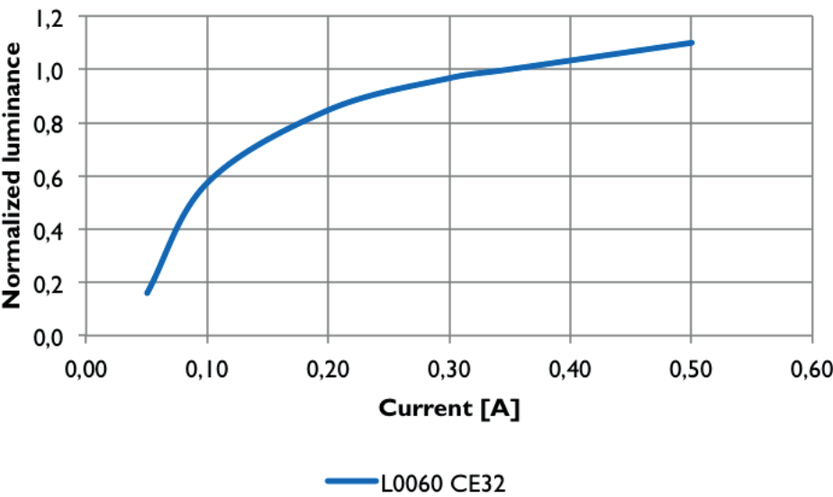
Luminance versus current
