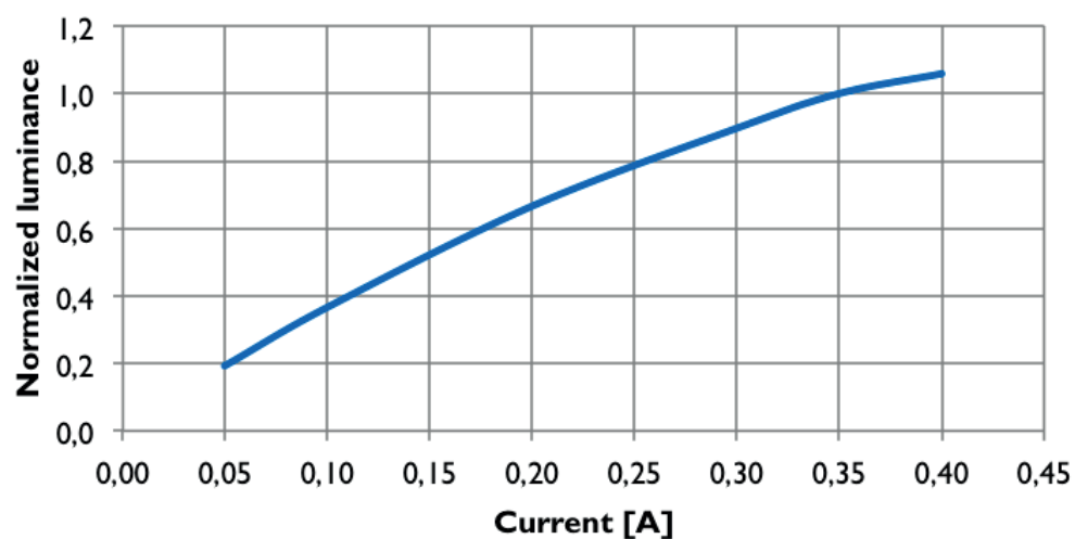
Luminance versus current
