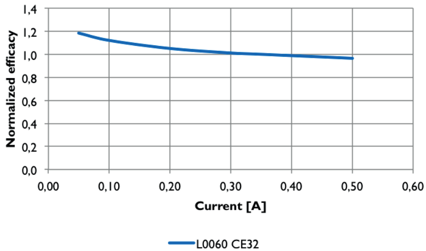
Luminous efficacy versus current density
