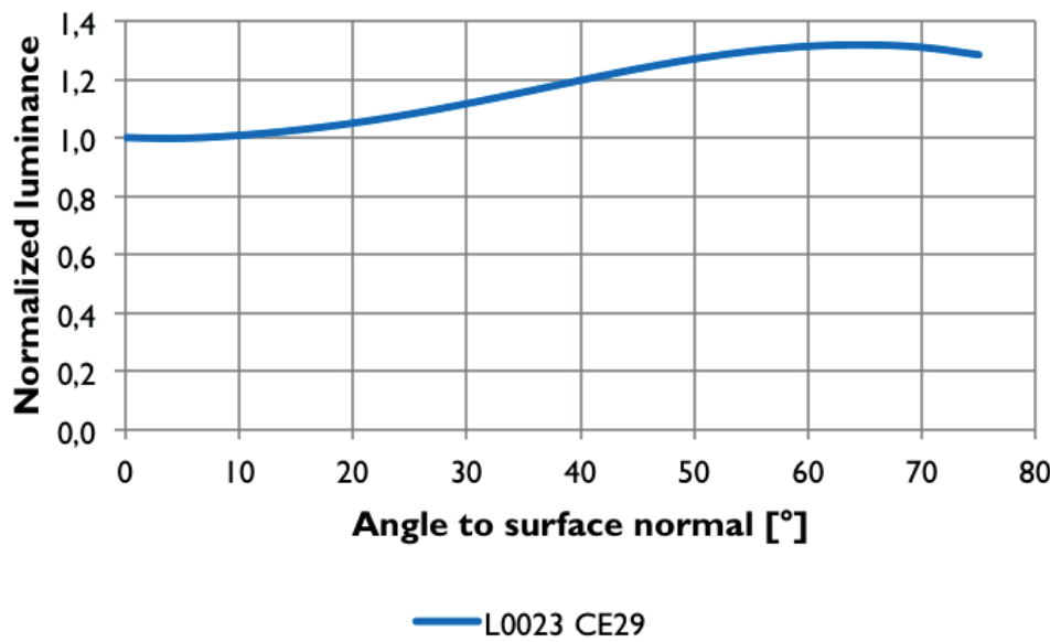
Luminance versus angle
