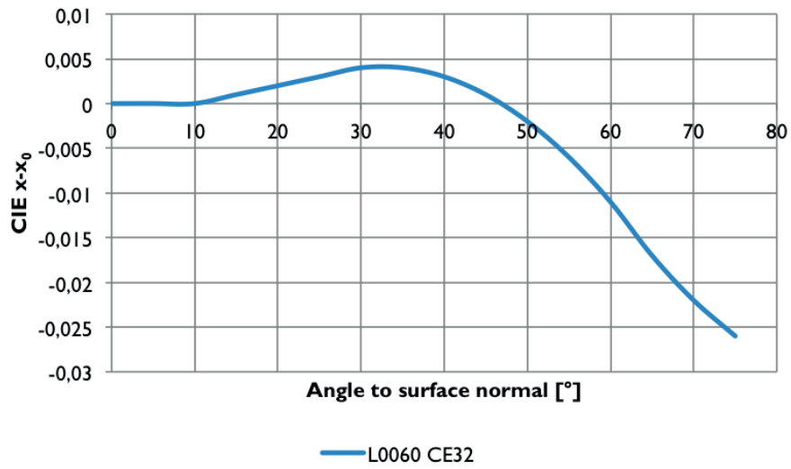
Color versus angle
