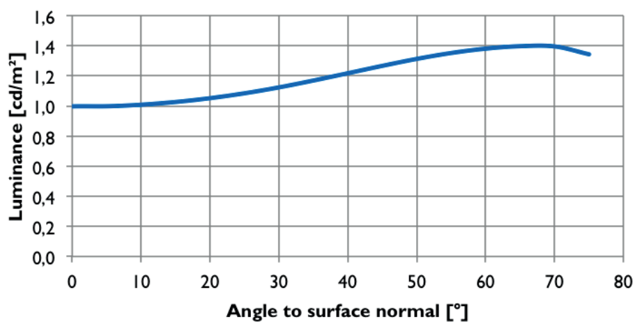
Luminance versus angle
