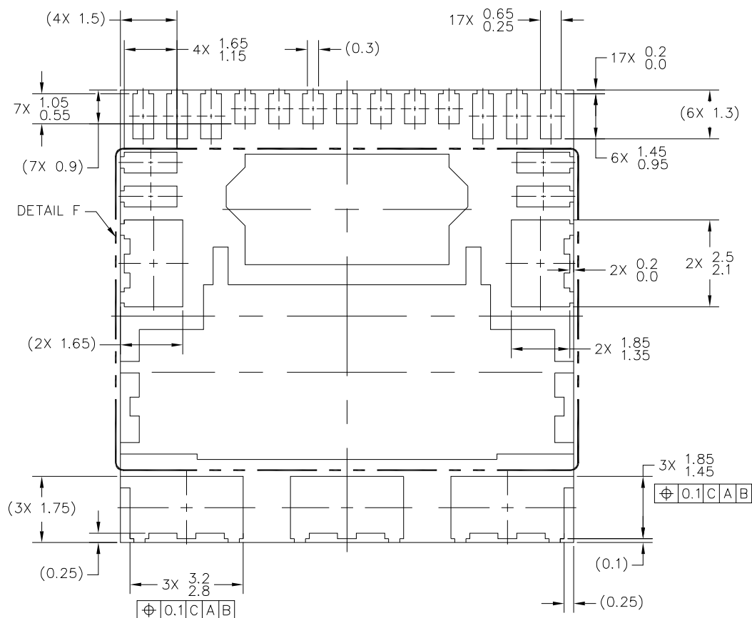
DETAIL E
