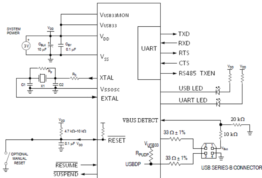
Figure 4. System connections working at 3 V
