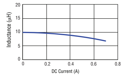
SRN2508A-100M
