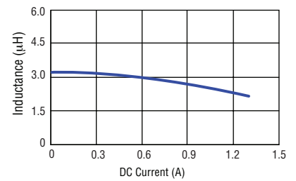
SRN2508A-3R3M
