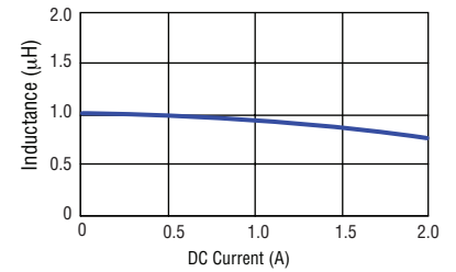
SRN2508A-1R0M
