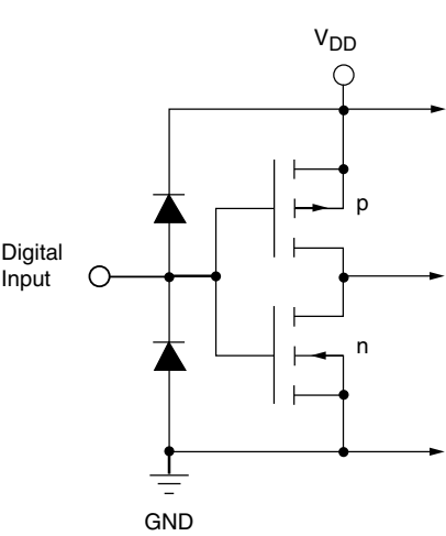
Figure 3. Equivalent Input Circuit
