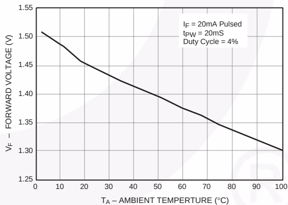
Fig. 6 Forward Voltage vs. Ambient Temperature
