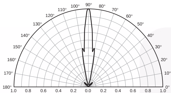
Fig. 7 Radiation Diagram
