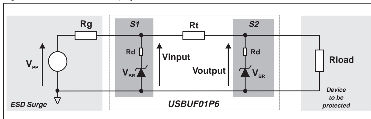
Fig. A5: USBUEF01P6 ESD clamping behavior
