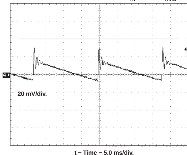
No Load Output Voltage Ripple, V_{IN} = 115 V_{RMS}
